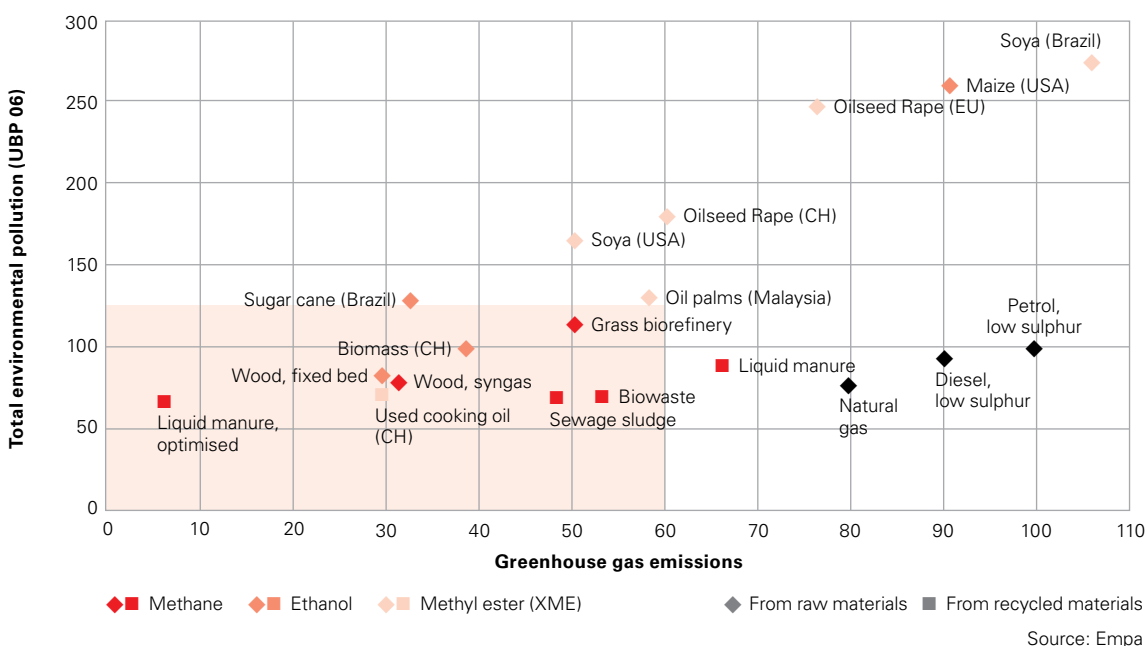
Figure 8. Greenhouse gas emissions and environmental pollution from biofuels compared to petrol. Fuels in the area underlaid in red meet the minimum requirements for mineral oil tax exemption, for greenhouse gas emissions and also for total environmental pollution.
