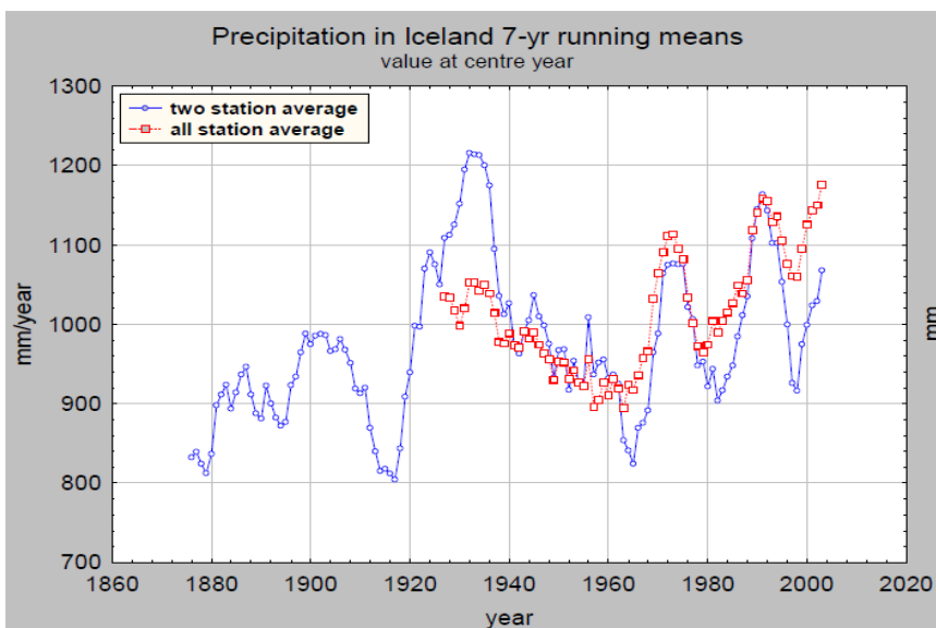
Fig. 3.14. : Annual precipitation in Iceland (7-yr running means)
