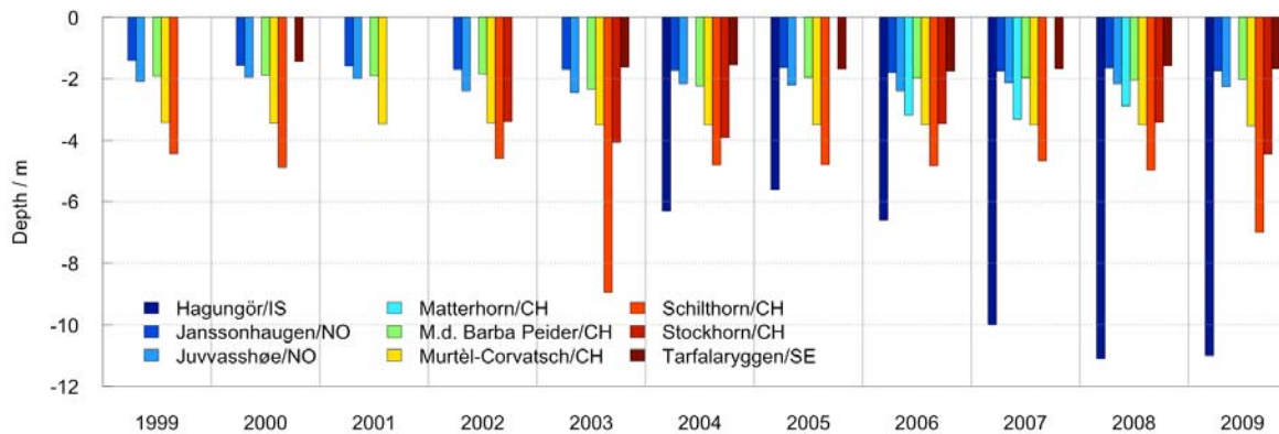
Figure 4.10: Maximum active layer thickness from different borehole sites in the Alps (Switzerland), Iceland, Norway and Svalbard (Janssonhaugen). The active layer is the upper layer of the ground, which is thawing in summer (and refreezing in winter).
