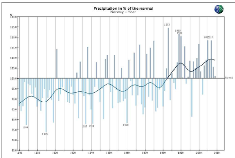
Fig.3.5a: Development of annual precipitation for Norwegian mainland (1900-2008) Source : met.no; 2009 Note: Bars show annual differences from the normal period 1961-1990; the curve is smoothed on a decadal scale
