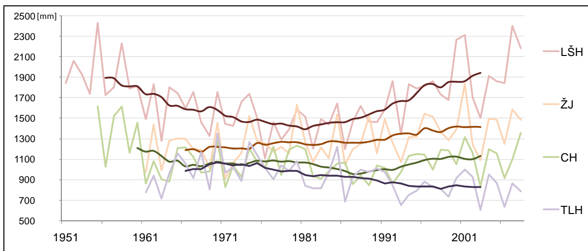
Figure 3.17: Yearly sums of daily precipitation totals and 11-year running averages from Lomnický štít (LŠH), Ždiar-Javorina (ŽJ), Chopok (CH) and Telgárt (TLH) stations Source : Stastny et al. (SHMU; 2010)
