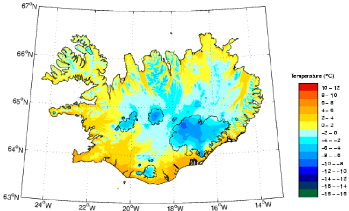
Figure 3.10: Annual mean temperatures in Iceland Source : http://www.vedur.is/vedurfar/vedurfarsmyndir/EV_DTO/ann.html
