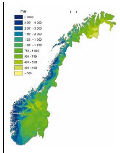
Fig.3.5b: Average annual precipitation in Norway 1979-2008 Source : met.no; 2009
