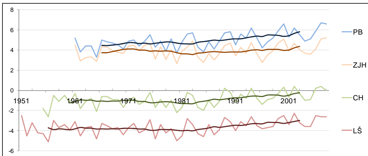
Figure 3.16: Yearly averages of mean daily temperatures (°C) and 11-year running averages from Podbanské (PB), Ždiar-Javorina (ZJH), Chopok (CH) and Lomnický štít (LŠ) stations Source: Stastny et al. ( SHMU; 2010)
