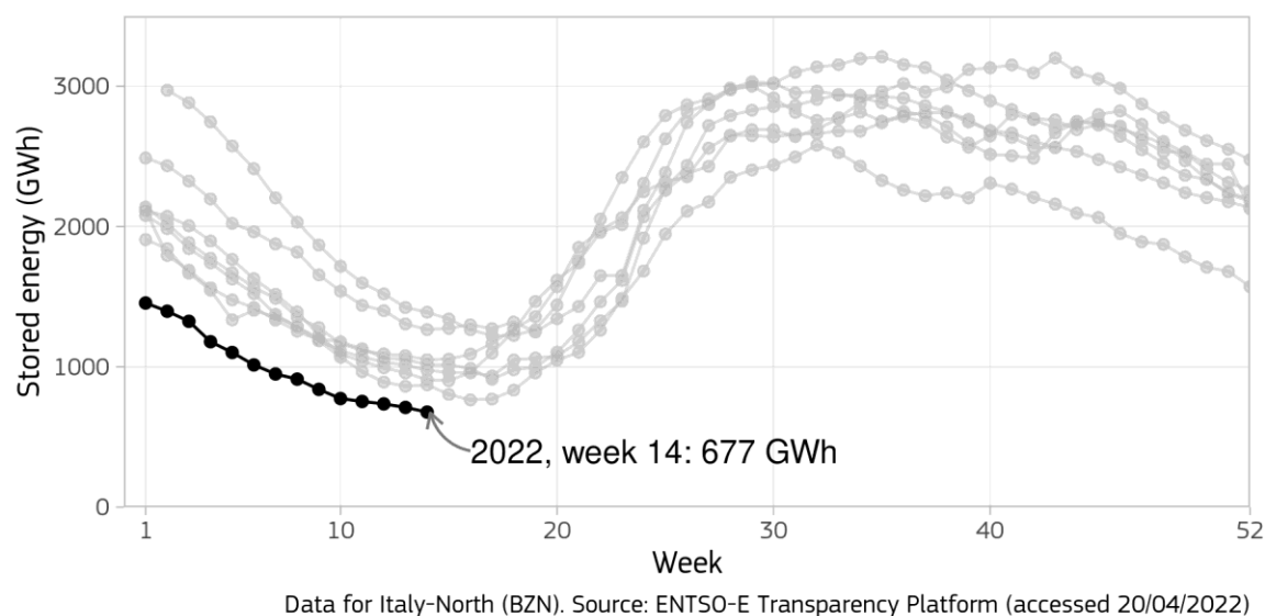
Figure 13: Hydropower storage levels in North of Italy for the period 2015–2022. Each grey line represents a specific year. The black line is associated with 2022. Source: ENTSO-E Transparency Platform.
