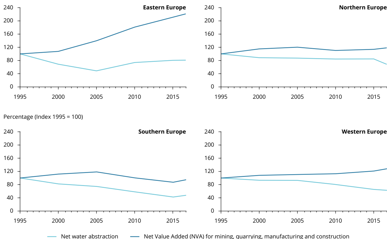
Figure 4.15 Comparison of regional trends in water consumption and economic growth in the industrial sector in Europe (EEA-38 and the UK), 1995-2017
