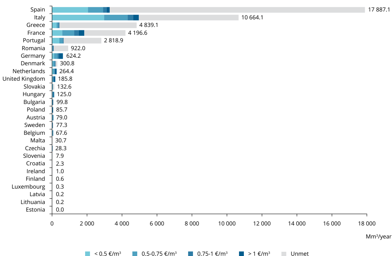
Figure 6.1 Water reuse potential per EU Member State (Mm 3 per year) for different levels of production cost
