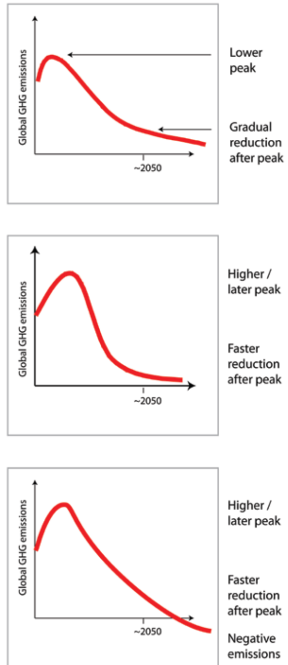
Figure A: Illustration of different pathway types for the same temperature increase. See Point 1 for explanation.
