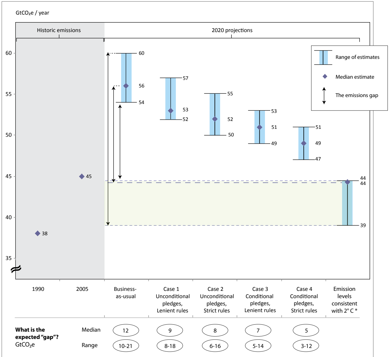
Figure C: Comparison of expected emissions in 2020 with the emission levels consistent with a “likely” chance of meeting the 2° C limit. The figure compares the expected emissions in 2020 resulting from the four pledge cases with the emission levels consistent with a “likely” chance of meeting the 2° C limit. The median estimates and range of estimates (20 th to 80 th percentile) are shown. The gap between expected emissions and the 2° C levels is given below in each case.
