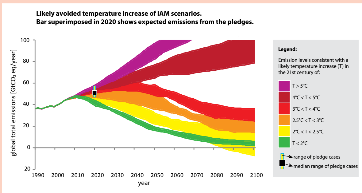
Figure B – Temperature increases associated with emission pathways and compared to the expected emissions from the pledges: Coloured bands show groups of IAM emission pathways that have approximately the same “likely” avoided temperature increase in the twenty-first century. Specifically the coloured bands show the 20th to 80th percentile range of the IAM pathways associated with those temperature increases. 15 Superimposed on top of the pathways is the range of estimated emissions resulting from the Copenhagen Accord pledges. The small black bar shows the range of median estimates from the four pledge cases. The thin blue bar represents the wider range of estimates associated with those four cases (the 20th to 80th percentile range).
