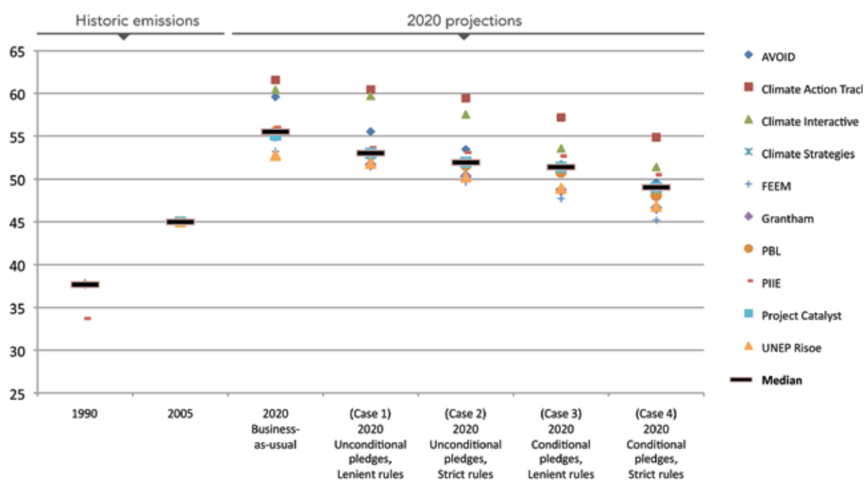
Figure 2. Global emissions resulting from the four pledge cases, as found by different modelling groups
